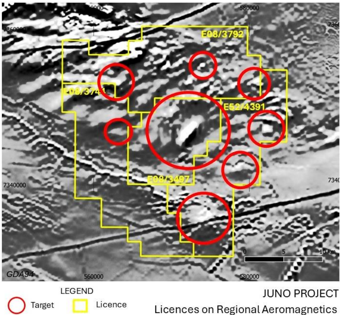
Figure 1 – New exploration licence application 08/3792, with existing licences and applications at the Juno Project, and targets on regional aeromagnetics (TMI 1VD).
